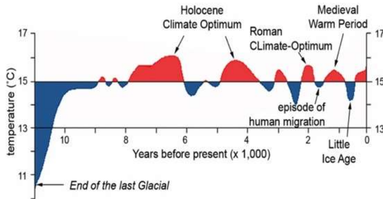
Northern Hemispheric temperature reconstruction for the past 10,000+ years
